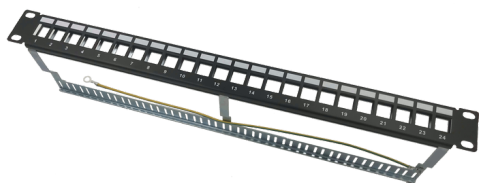
Panneau 19", 1U, sans insert 19" Panel, 1U, without Inserts
